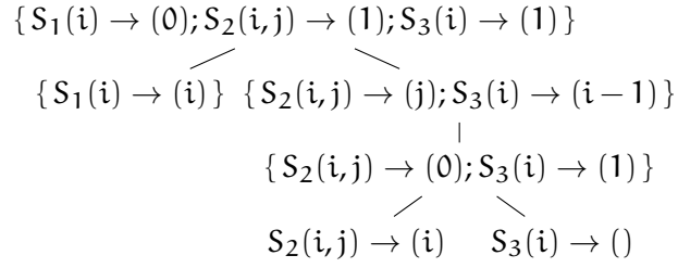
Figure 43: Band forest representation of the schedule in Figure 42
