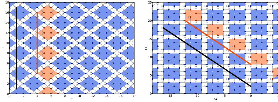
Figure 21: Symmetric dependences &amp; square tiling (original/transformed)
