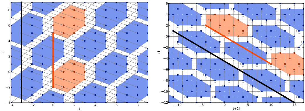
Figure 27: Hexagonal-tiling (original/transformed)
