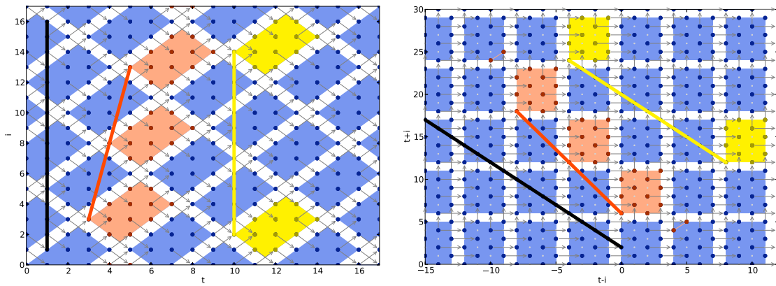
Figure 22: Symmetric dependences &amp; non-square tiling (original/transformed)
