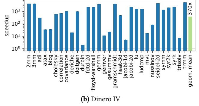
Figure 15. Speedup of HayStack compared to PolyCache and Dinero for the PolyBench 3.2 and 4.2.1 kernels, respectively.
