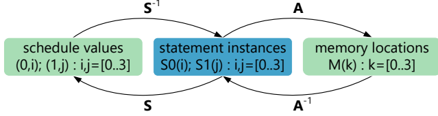
Figure 3. The statement instances and the related schedule values (schedule \mathbf{S} ) and memory accesses (access map \mathbf{A} ) are sufficient to compute the cache misses of a program.
